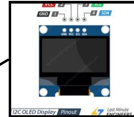
0.96inch OLED Display
