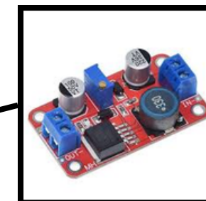
XL6019 Step-up Converter
